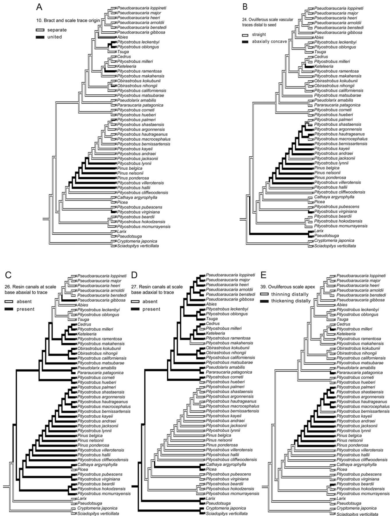
FIG. 5. Parsimony character state reconstructions for ovulate cone characteristics used to delimit Pinus from Pityostrobus . A. Bract and scale trace origin (character 10) separate (white) or united (black). B. Ovuliferous scale vascular trace transverse shape distal to seed (character 24) straight (white) or abaxially concave (black). C. Resin canals abaxial to ovuliferous scales at scale base (character 26) absent (white) or present (black). D. Resin canals adaxial to ovuliferous scales at scale base (character 27) absent (white) or present (black). E. Ovuliferous scale apex (character 39) thinning distally (white) or thickening distally (black). Taxa with polymorphic states are half black and half white.
