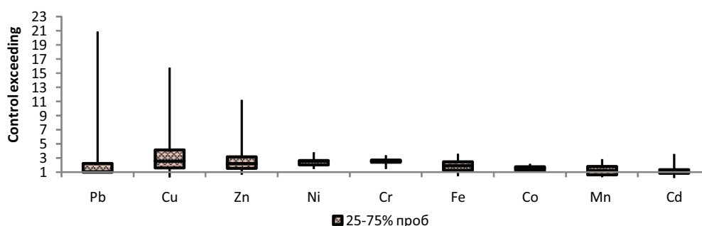
Figure 2. Heavy metals in soils of Tyumen exceeding the control in 2017 to 2020. Vertical lines indicate first and forth quartile, and horizontal line inside the box is median.
